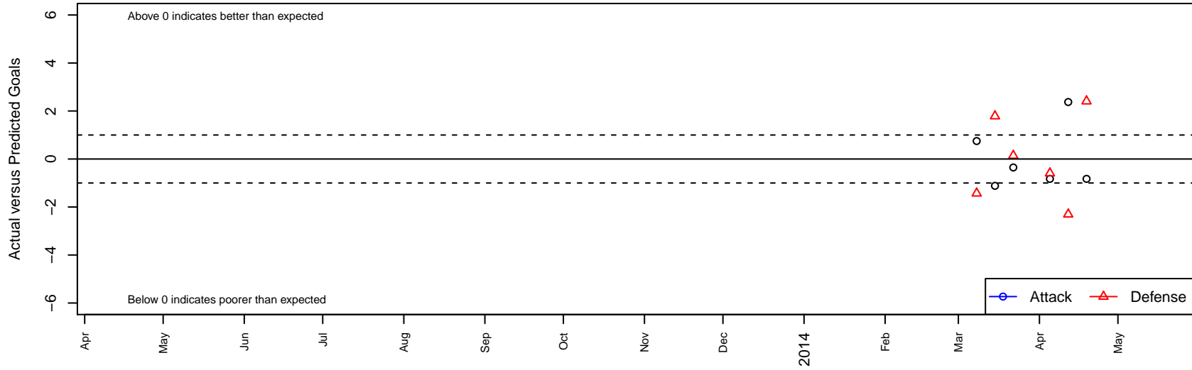
Tri City B00 Dots are actual minus expected GF (blue circles) and GA (red triangles). Blue line is smoothed change in attack strength. Red is smoothed change in defense strength.
